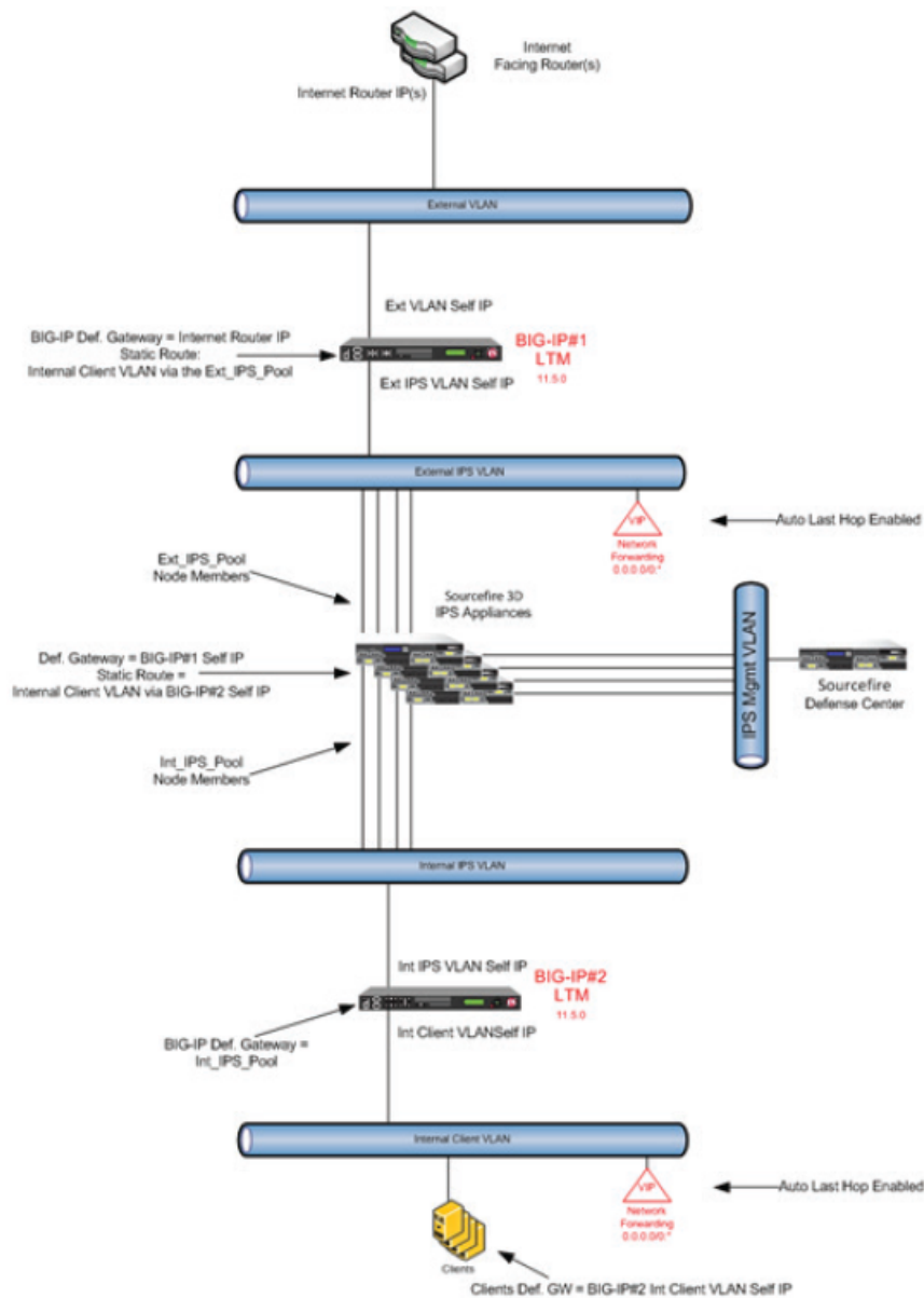
Figure 24: Egress Access Network Topology
